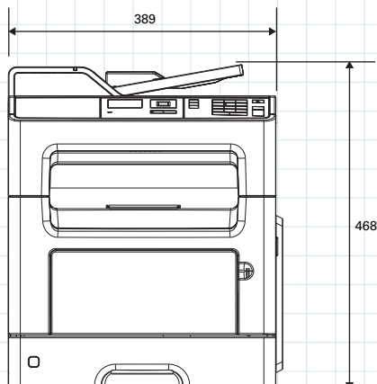
Front View bizhub 3320
